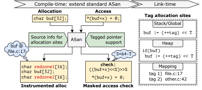
Figure 3: Overview of TagASan’s instrumentation.
